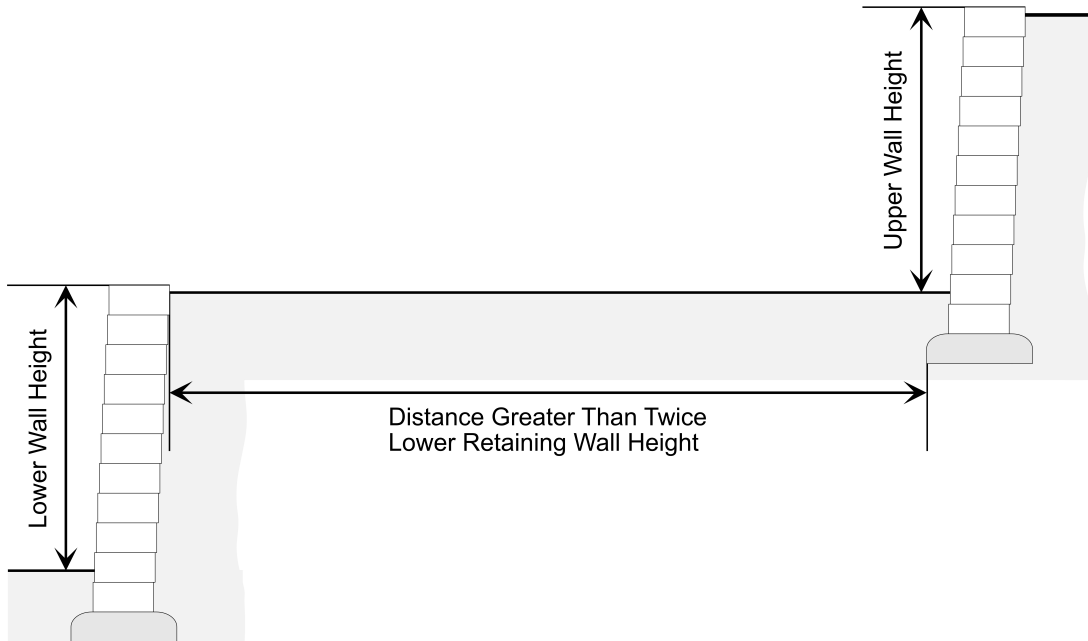
Figure 3-2: Measuring Retaining Wall Height
