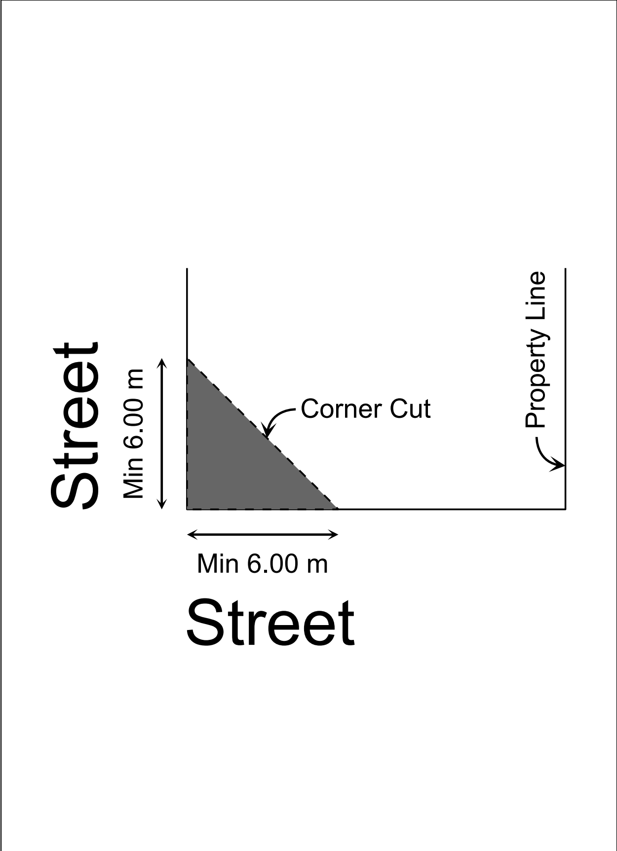
Figure 3-3: Corner Cut for Traffic Sight Lines
