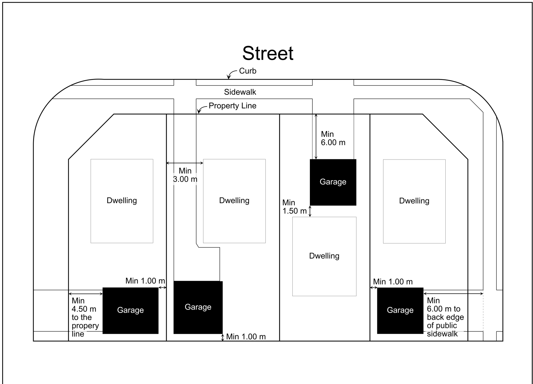
Figure 3-5: Detached Garage Setbacks
