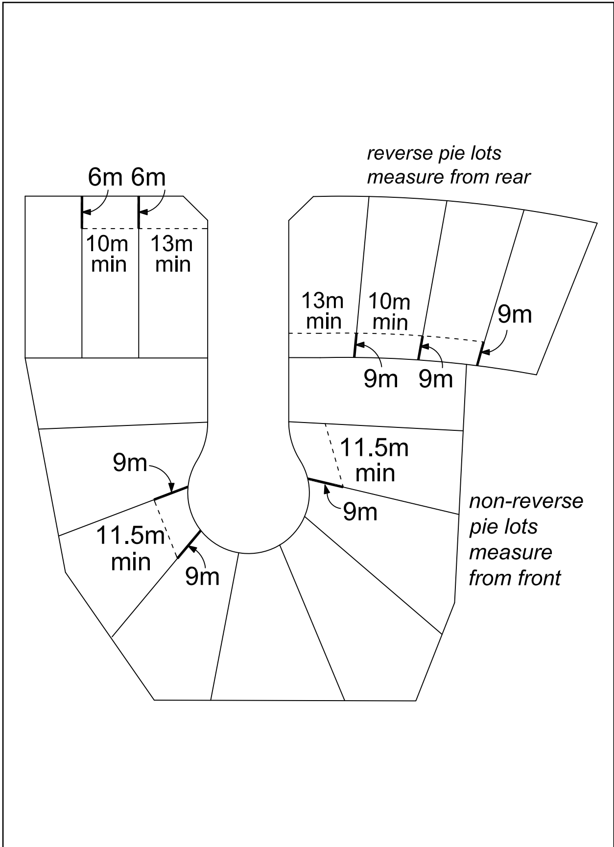
Figure 3-7: Lot Widths
