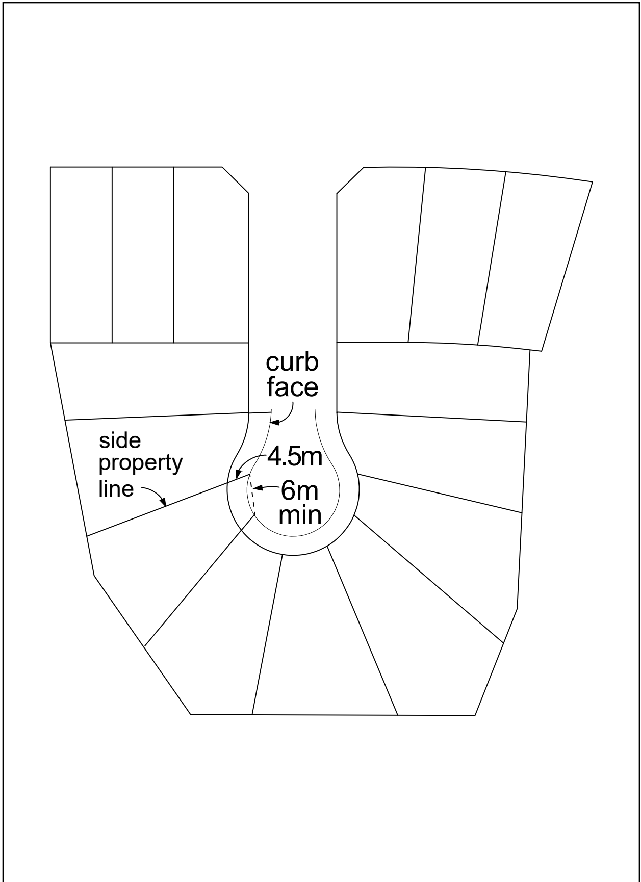
Figure 3-8: Curb Frontage Requirements for Pie Shaped Lots
