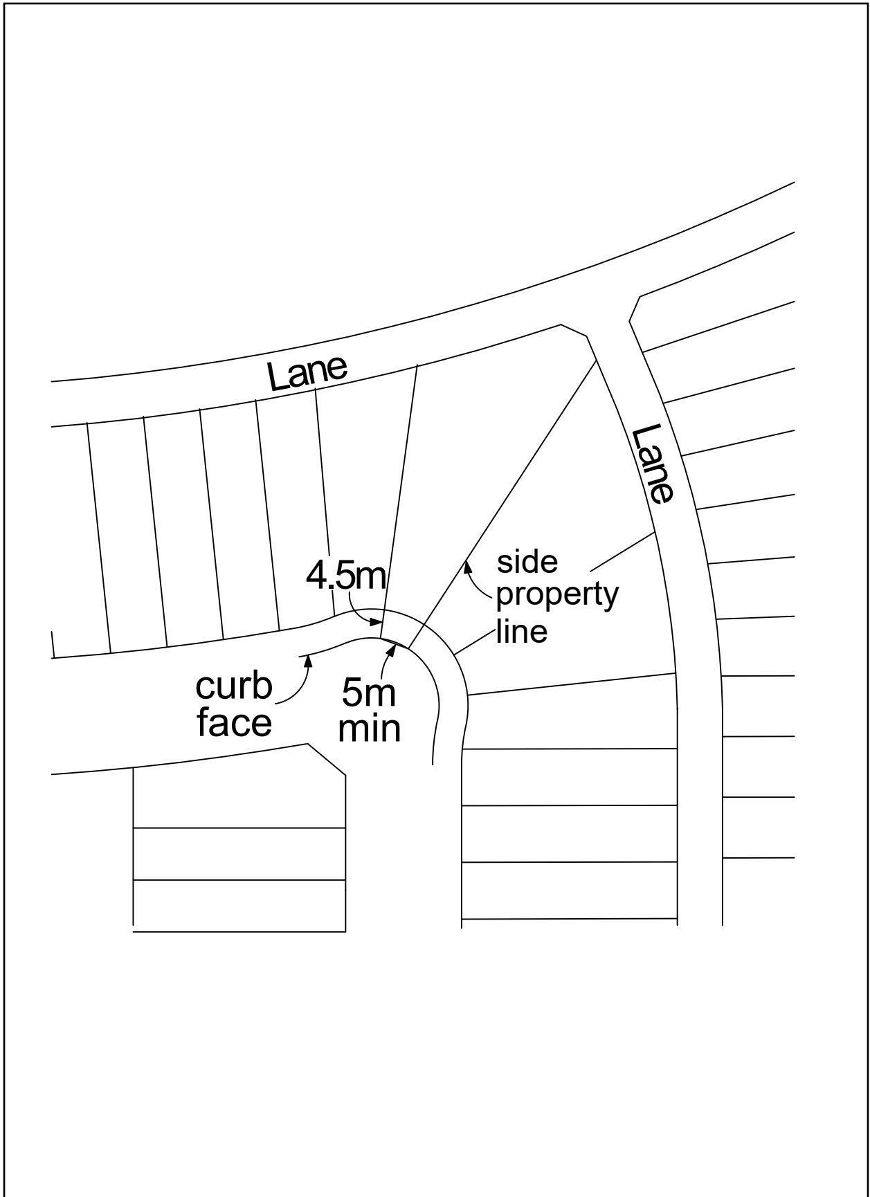
Figure 3-9: Curb Frontage Requirements for Rear Lane Access
