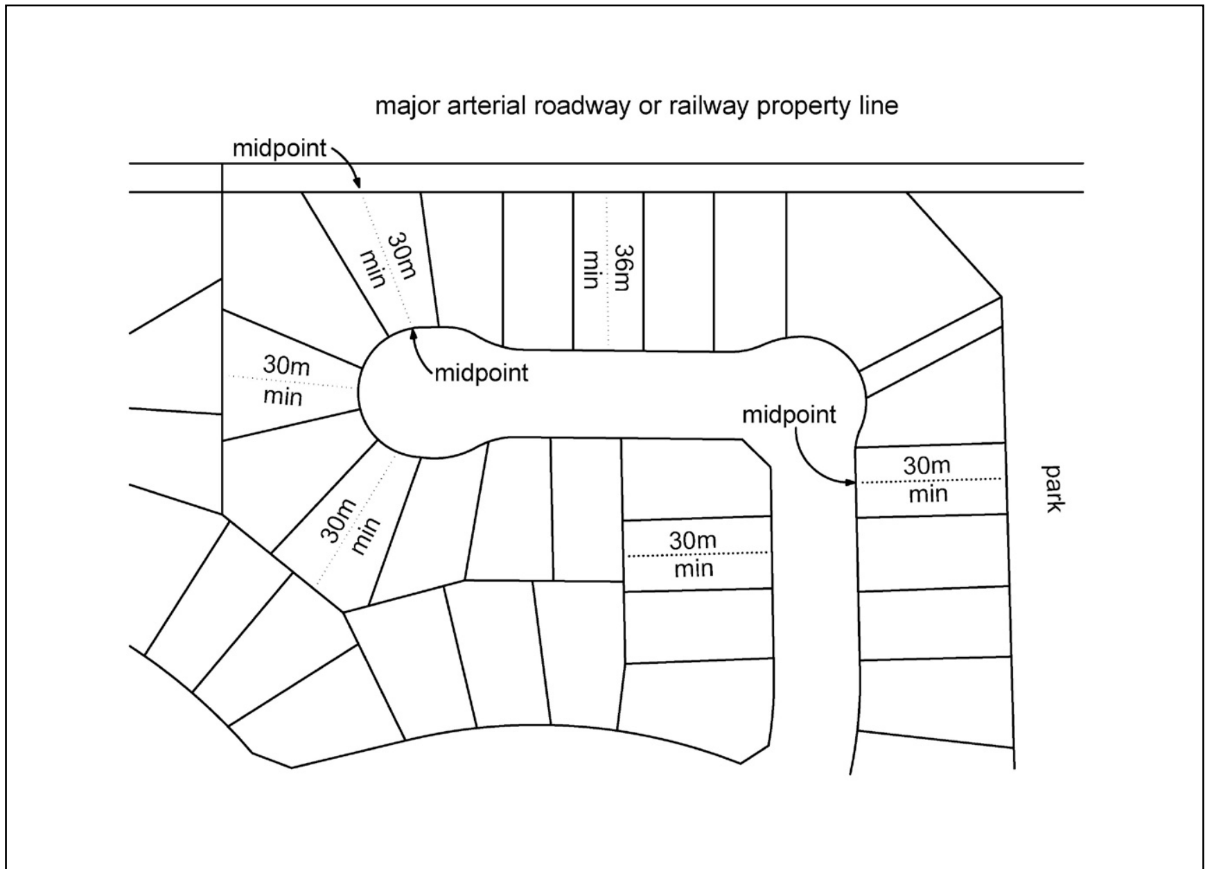
Figure 3-10: Lot Depth Requirements
