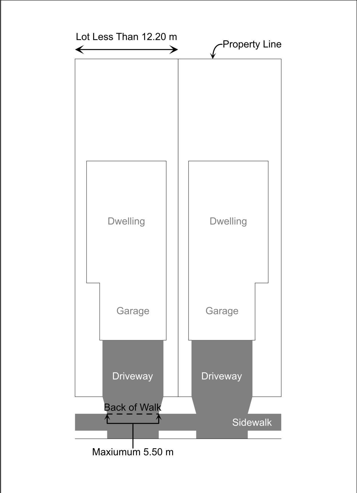
Figure 3-12: Measuring Lots Less than 12.20 m Wide
