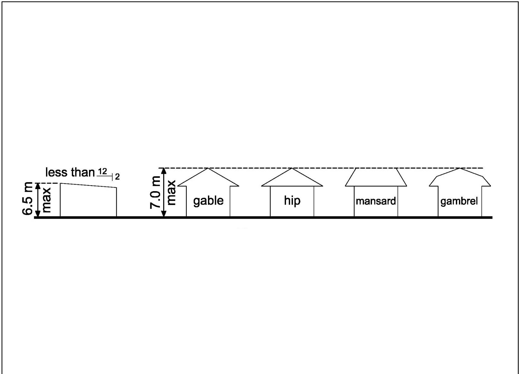
Figure 3-13: Maximum Height for Detached Garage with Garage Suite
