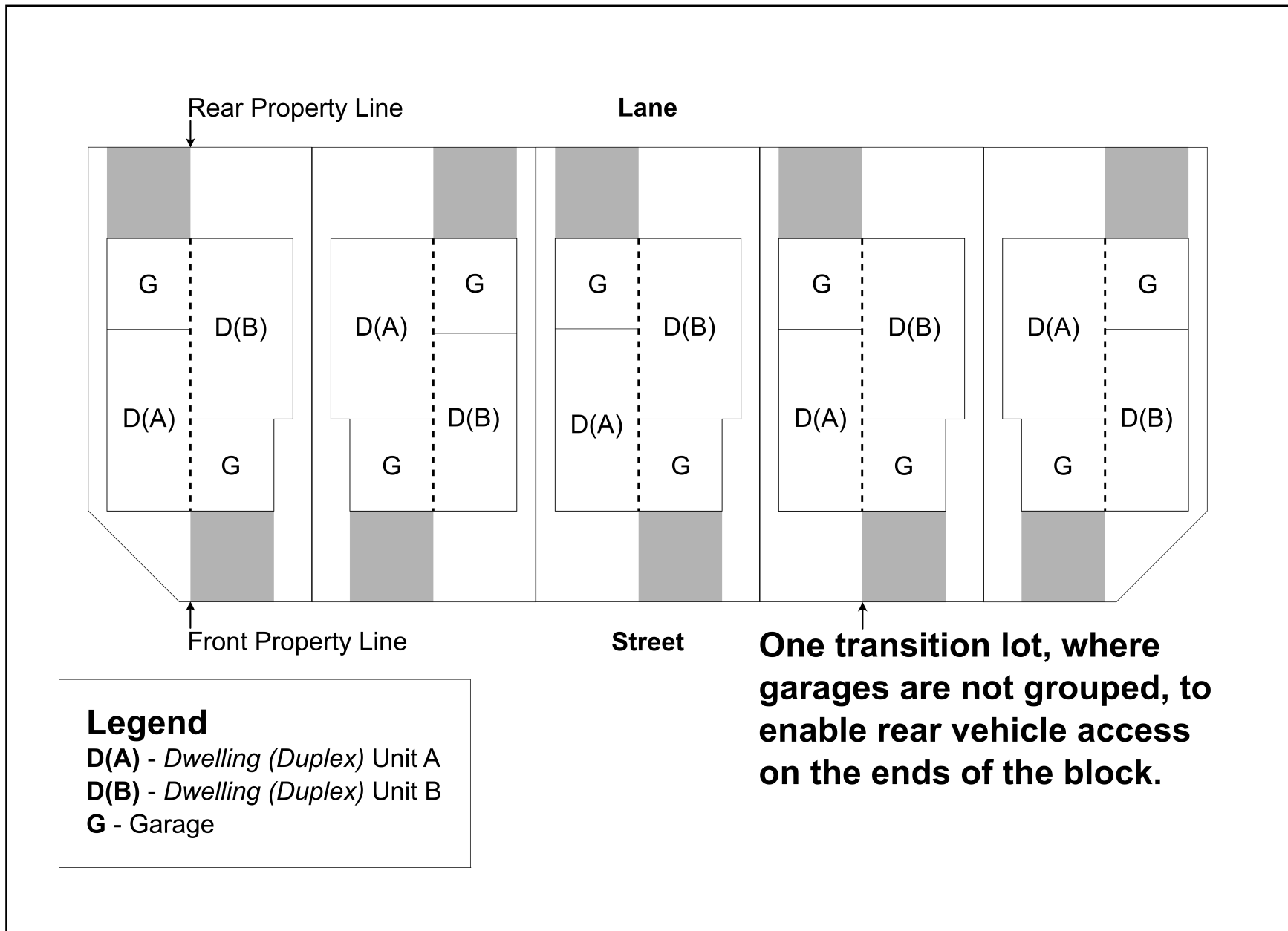
Figure 5-4: Grouping of Vehicular Access on Adjacent Lots for a Block of Dwelling (Duplex)
